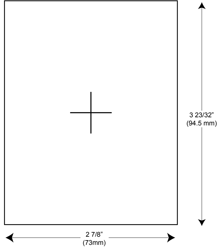
Point Pad Flush Mount Template Use U-Clamp to secure control switch
